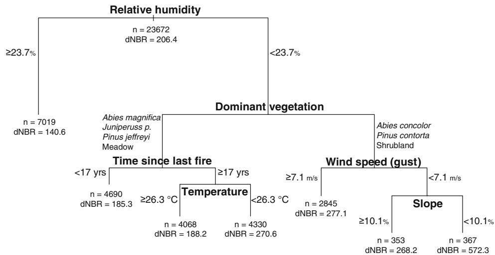
Fig. 5 Regression tree explaining the spatial distribution of differenced Normalized Burn Ratio (dNBR) values throughout the Hoover fire. The number of pixels, along with the average dNBR, in the resulting group is reported
