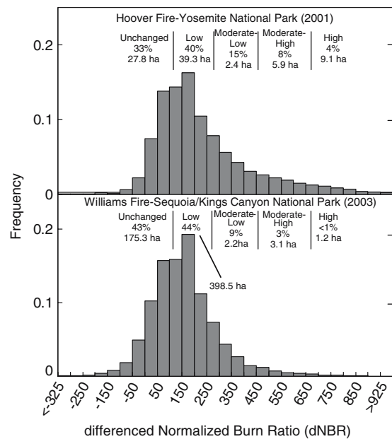
Fig. 4 Frequency distributions for differenced Normalized Burn Ratio values for the Hoover and Williams fires, along with the proportion of pixels and area-weighted mean patch size by fire severity rating class for each fire. The fire severity classes are based on Key and Benson (2005)
