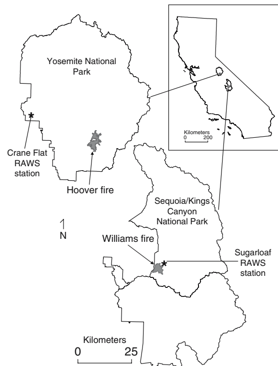
Fig. 1 Locations of the Hoover (Yosemite NP) and Williams (Sequoia/Kings NP) fires, California, USA
