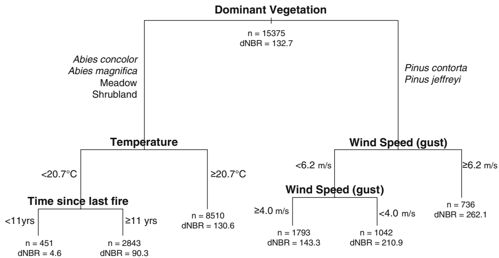
Fig. 6 Regression tree explaining the spatial distribution of differenced Normalized Burn Ratio (dNBR) values throughout the Williams fire. The tree is drawn and labeled as in Fig. 5. The total R^2 for the tree is 12%
